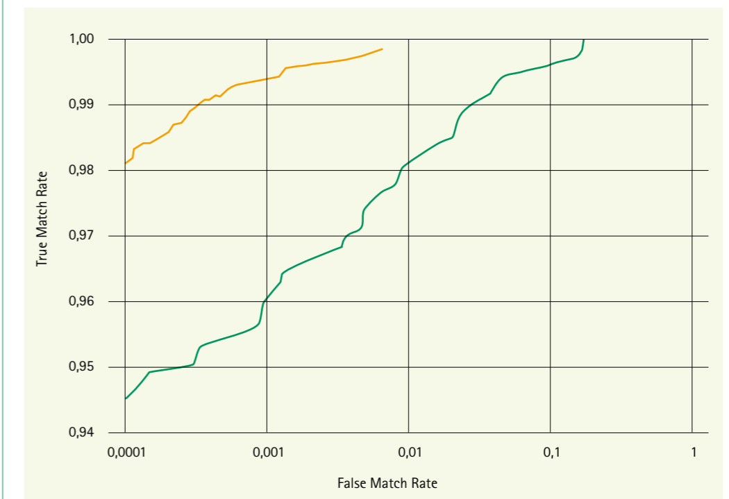
Verification performance in Grayscale FERET Duplicate I Test
